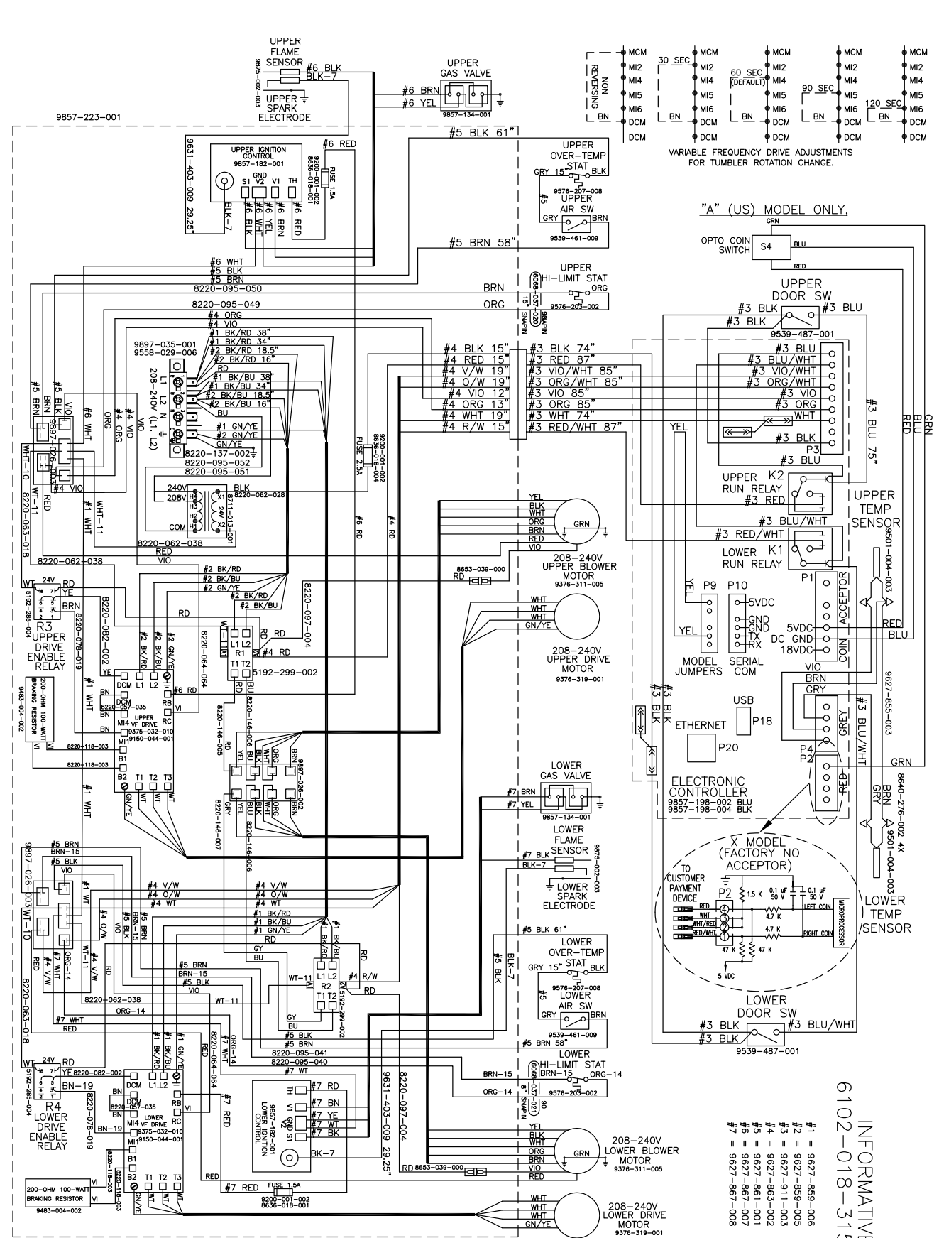
9506-790-001A WIRING DIAGRAM DC50X2NC-11EC_R
