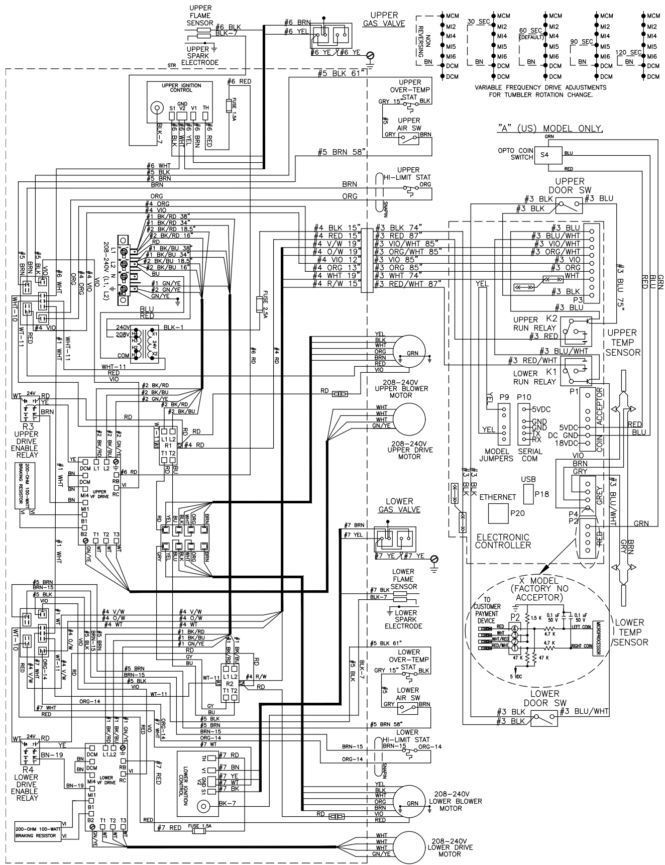
9506-790-001B WIRING DIAGRAM DC50X2NC-11EC_R
