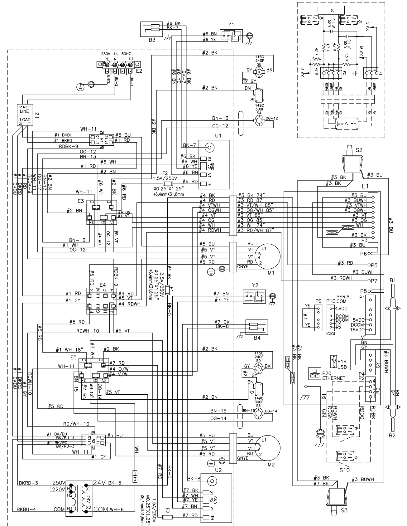
9506-646-001A WIRING DIAGRAM DC30X2N-59CC-X-
